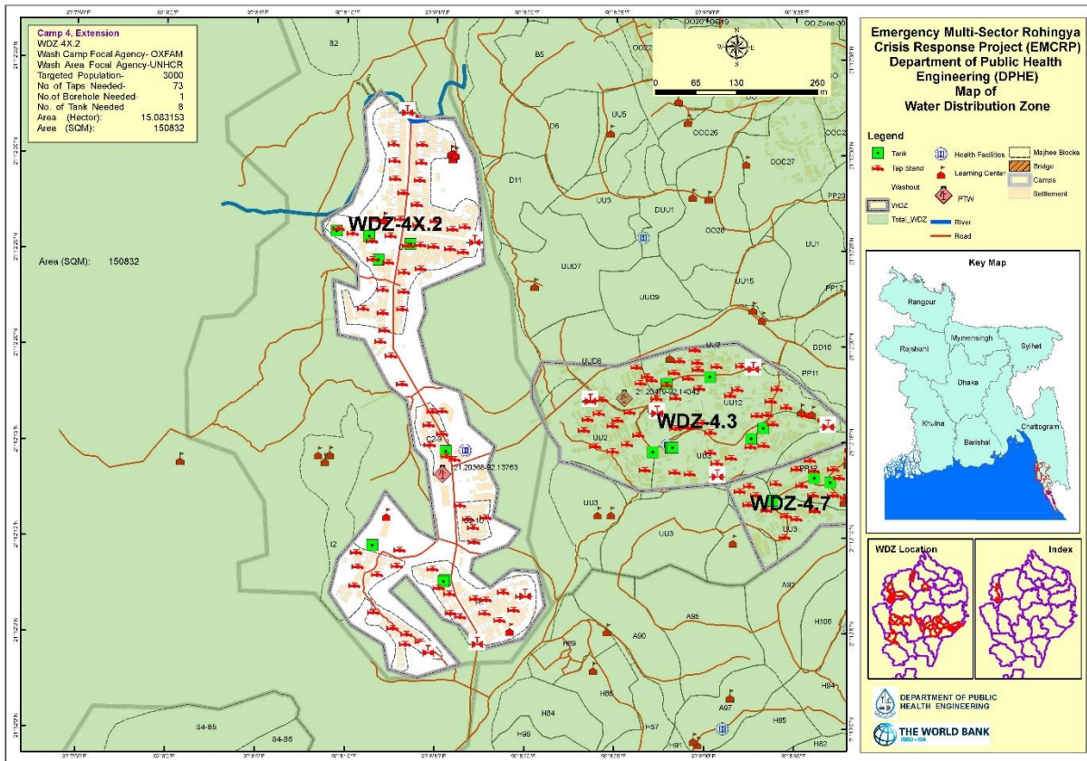
Map-2: Pipe Network Information Map of Water Distribution Zone (WDZ-04 extension.02)
